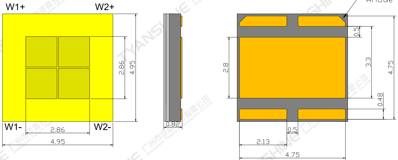
Top view
